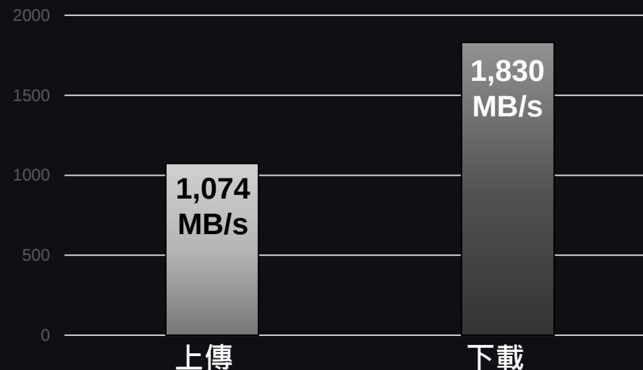
2 x 10GbE Windows 檔案拖拉 (10GB)
